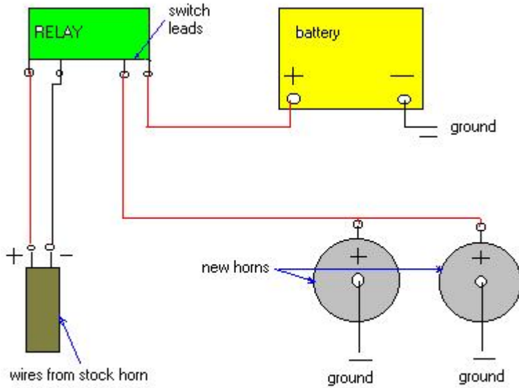
VOLUSIA HORN CIRCUIT
