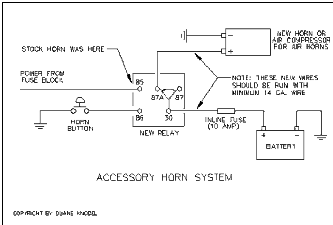
VOLUSIA HORN CIRCUIT
